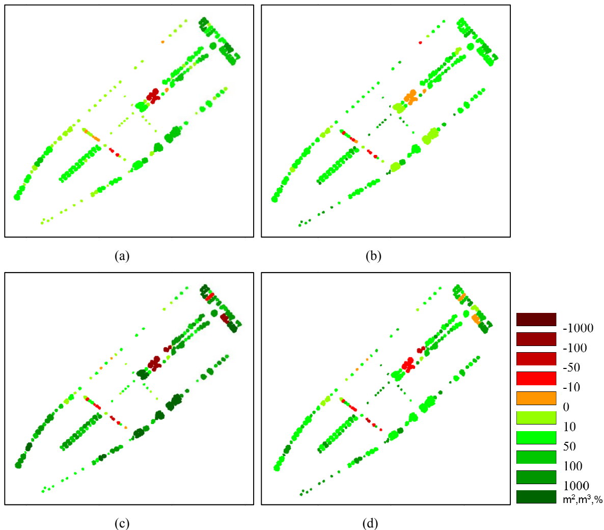
Figure 8. Change detection results (2008.03-2010.04), (a) area change ( m^2 ), (b) area change ratio (%), (c) volume change ( m^3 ), (d) volume change ratio (%).
